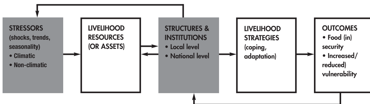
FIGURE 1: CONCEPTUAL FRAMEWORK
